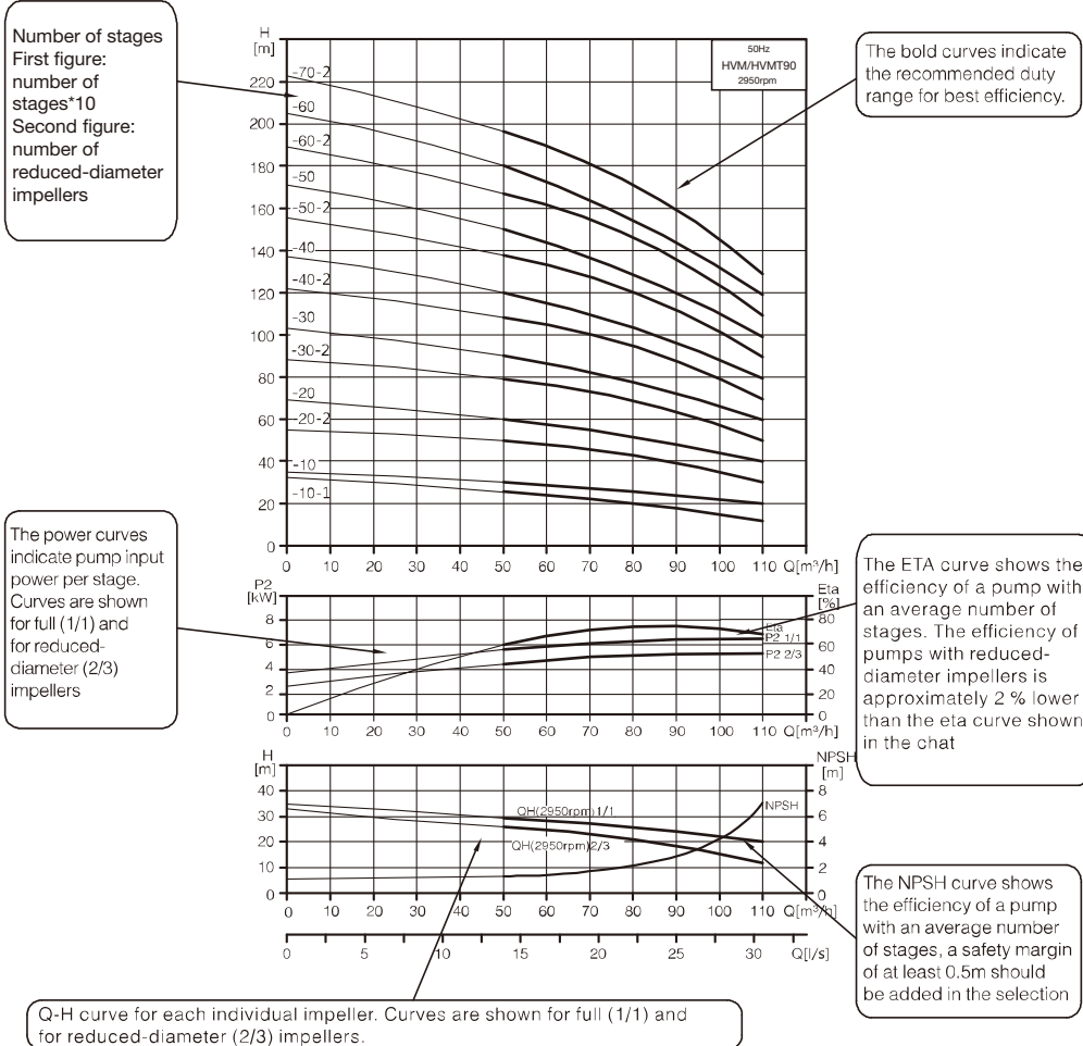
Performance curve
